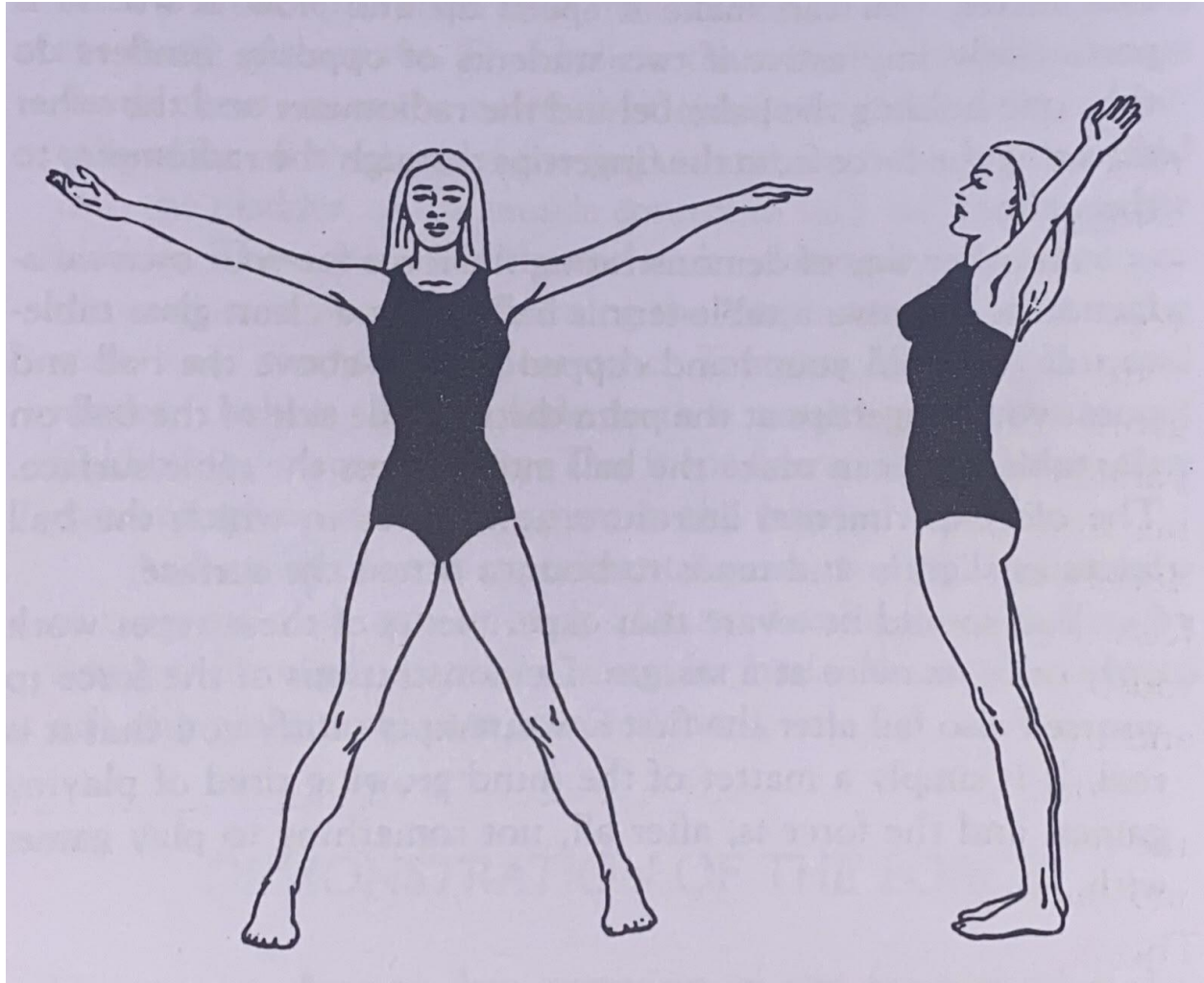
Figure 5. Star position
